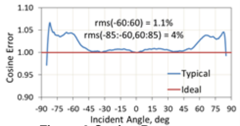
Figure 3 Cosine Response
