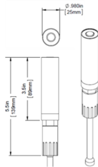
Figure 5 Dimensions
