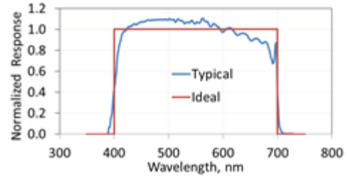
Figure 2 Spectral Response
